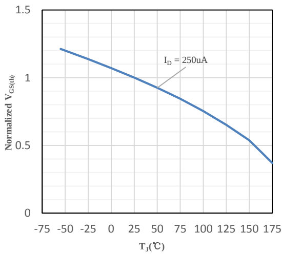
Fig 11 Normalized V_{GS(th)} vs T_J
