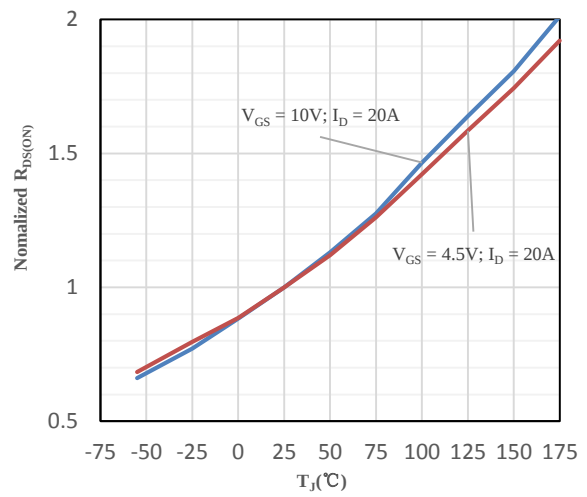
Fig 10 Normalized R_{DS(ON)} vs T_J
