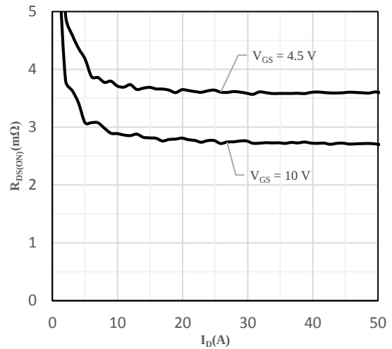
Fig 4 On-Resistance vs. Drain Current
