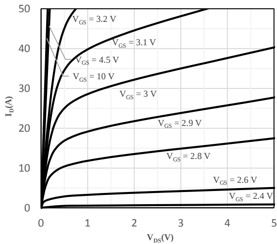
Fig 3 Output Characteristics
