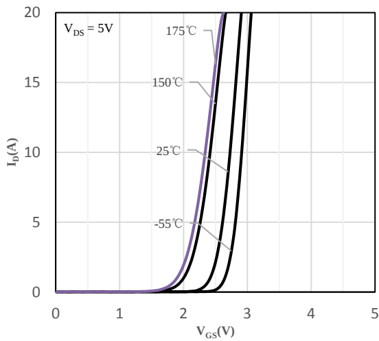
Fig 9 Transfer Characteristics
