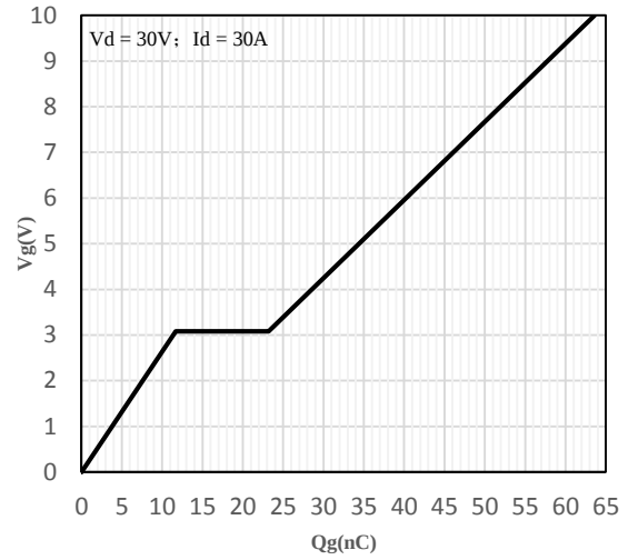
Fig 8 Gate-Charge Characteristics
