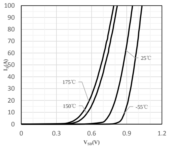
Fig 6 Body-Diode Characteristics
