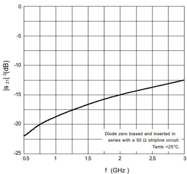
Fig.5 Isolation ( |s_{21}|^2 ) of the diode in off-state as a function of frequency; typical values.
