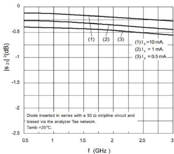
Fig.4 Insertion loss ( |S_{21}|^2 ) of the diode in on-state as a function of frequency; typical values.
